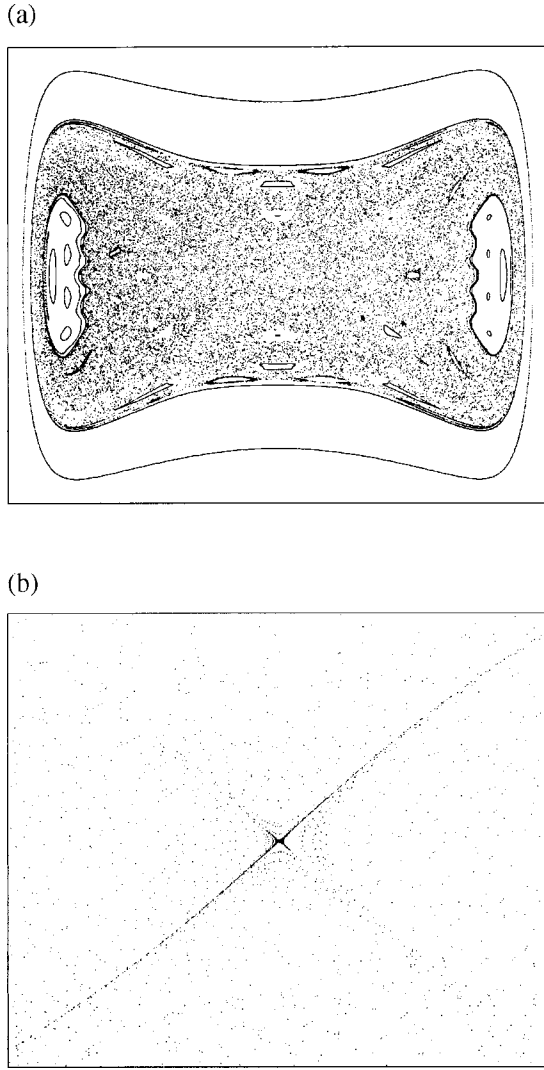
FIG. 3. (a) x=0 Poincaré section ( y, p_y axes) for the elliptic potential, Eq. (62), with \lambda = 53/\pi and k = 7.43 . (b) Zoom of the central region where the y = p_y = 0 long straight-line orbit is unstable.
