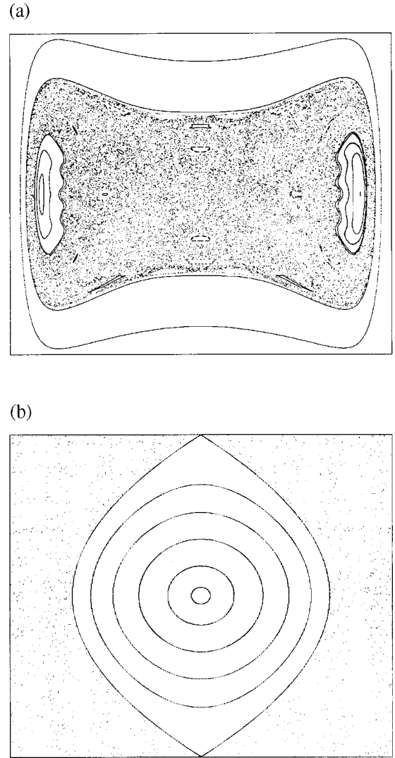
FIG. 4. (a) x=0 Poincaré section ( y, p_y axes) for the elliptic potential, Eq. (62), with \lambda = 53/\pi and k = 7.44 . (b) Zoom of the central region where the y = p_y = 0 long straight-line orbit is now stable.
