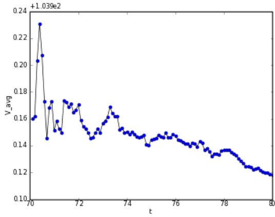
Figure 19: Temperature, Pressure, Volume, Polarization verse time for MD simulation of LiNbO3 at target temperature T=1900 K (new080514).
