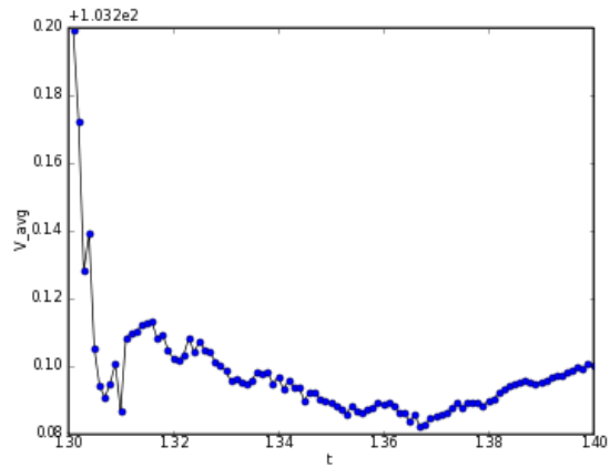
Figure 8: Temperature, Pressure, Volume, Polarization verse time for MD simulation of LiNbO3 at target temperature T=800 K (new080514).
