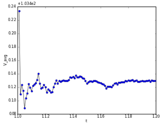
Figure 11: Temperature, Pressure, Volume, Polarization verse time for MD simulation of LiNbO3 at target temperature T=1100 K (new080514).
