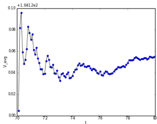
Figure 18: Temperature, Pressure, Volume, Polarization verse time for MD simulation of LiNbO3 at target temperature T=1800 K (new080514).
