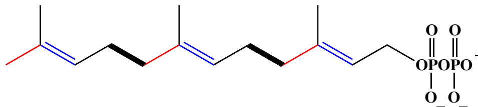
farnesyl pyrophosphate (FPP)
