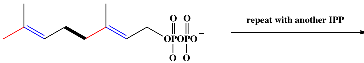
geranyl pyrophosphate (GPP)
