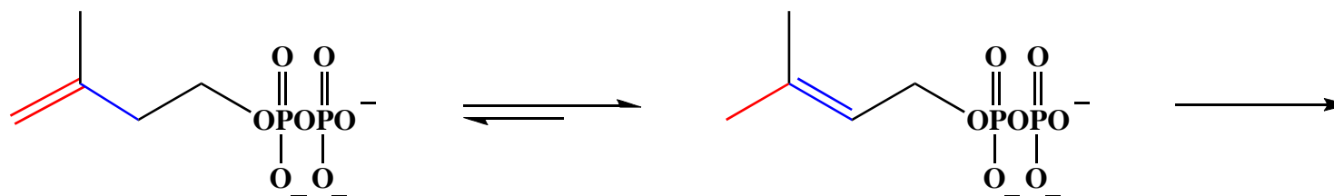
isopentenyl pyrophosphate (IPP)
