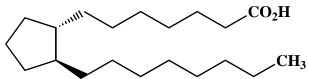
Prostanoic acid
