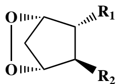
PGG, PGH
