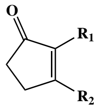
PGB
