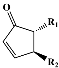
PGA
