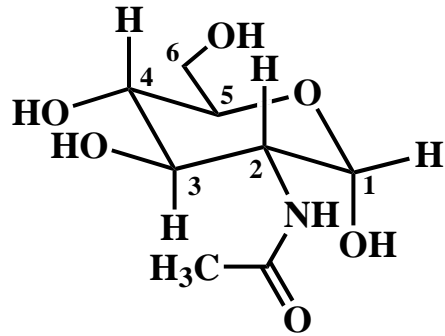
N -acetylglucosamine
