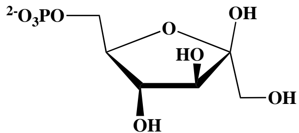
fructose-6-phosphate
