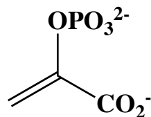
phosphoenolpyruvate
