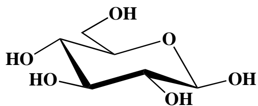
glucose
