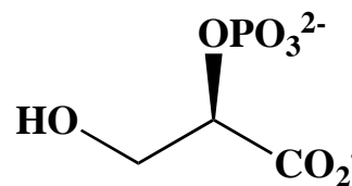
2-phosphoglycerate
