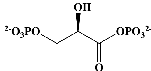
1,3-bisphosphoglycerate
