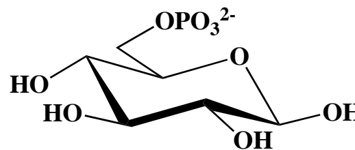
glucose-6-phosphate
