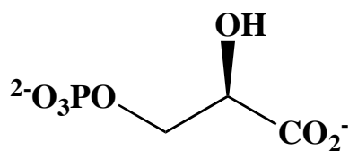
3-phosphoglycerate
