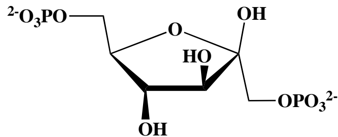
fructose-1,6-bisphosphate
