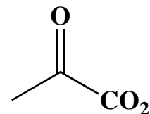
pyruvate
