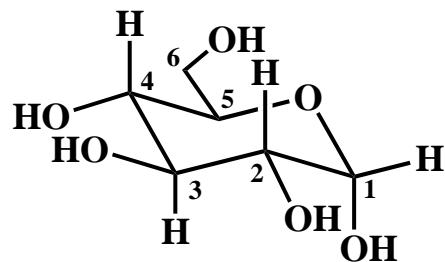
\alpha -D-glucopyranose
