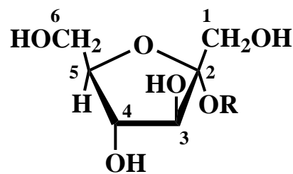
an alkyl \alpha -D-fructofuranoside
