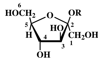
an alkyl \beta -D-fructofuranoside
