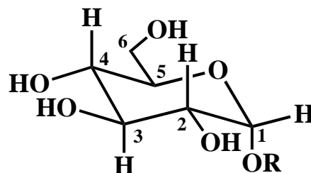
an alkyl \alpha -D-glucopyranoside
