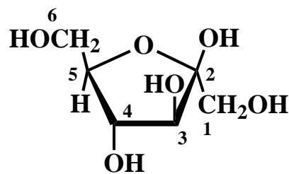
\beta -D-fructofuranose
