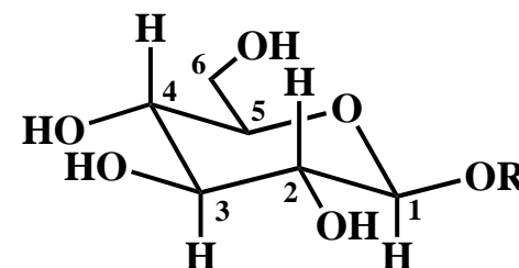
an alkyl \beta -D-glucopyranoside
