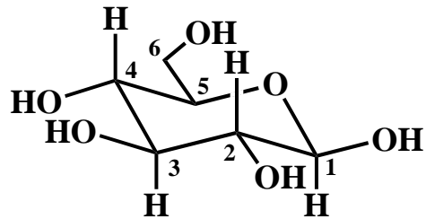
\beta -D-glucopyranose
