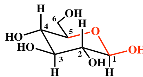
\beta -D-glucopyranose
