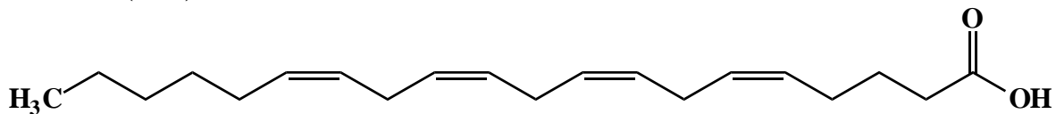
arachidonic acid (20:4)
