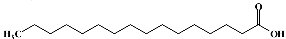
palmitic acid (16:0)
