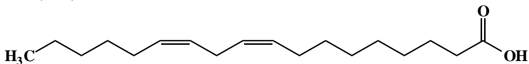
linoleic acid (18:2)
