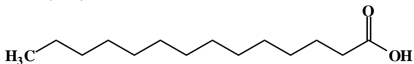
myristic acid (14:0)
