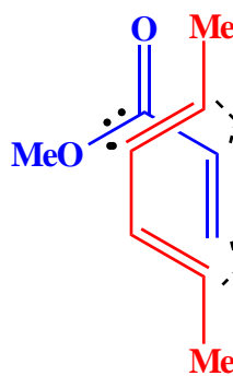
Endo transition state (looking from above)
