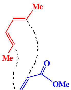
Exo transition state (looking from the side)
