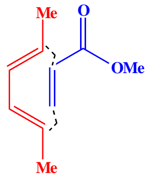
Exo transition state (looking from above)
