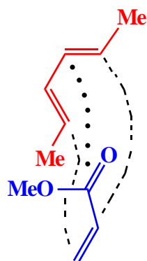
Endo transition state (looking from the side)
