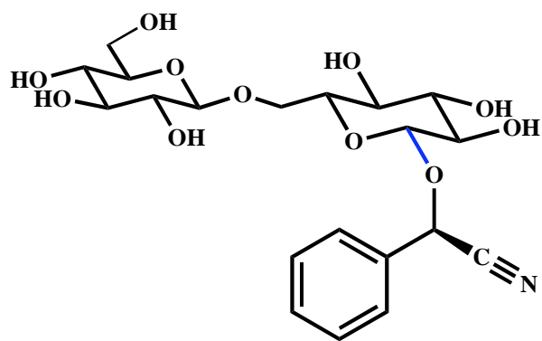
amygdalin
