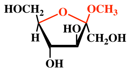
\alpha \beta -D-fructoside
