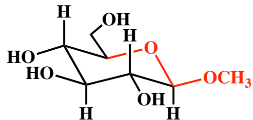
\alpha \beta -D-glucoside
