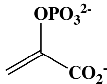
phosphoenolpyruvate
