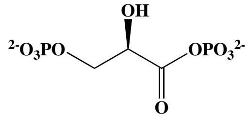
1,3-bisphosphoglycerate
