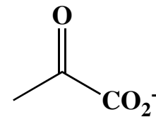
pyruvate
