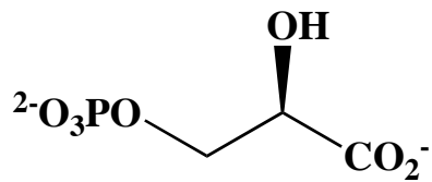
3-phosphoglycerate
