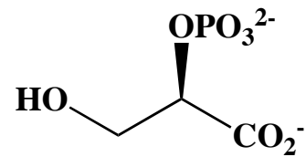
2-phosphoglycerate
