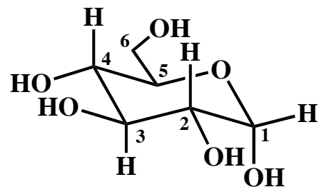
\alpha -D-glucopyranose
