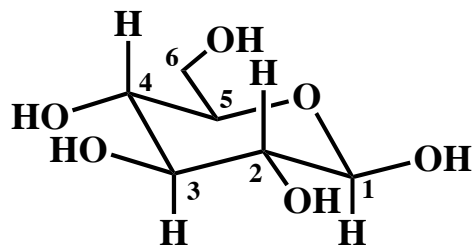
\beta -D-glucopyranose
