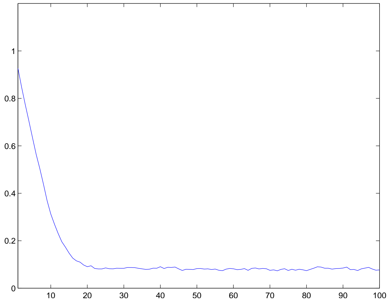
Individual run with N = 100 and \sigma = 5 averaged over 70 runs
