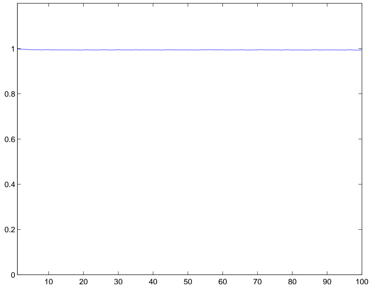
Individual run with N = 100 and \sigma = 0.75 averaged over 70 runs
