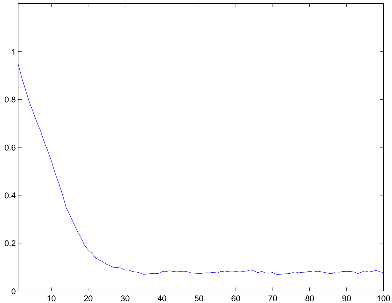
Individual run with N = 100 and \sigma = 4.25 averaged over 70 runs
