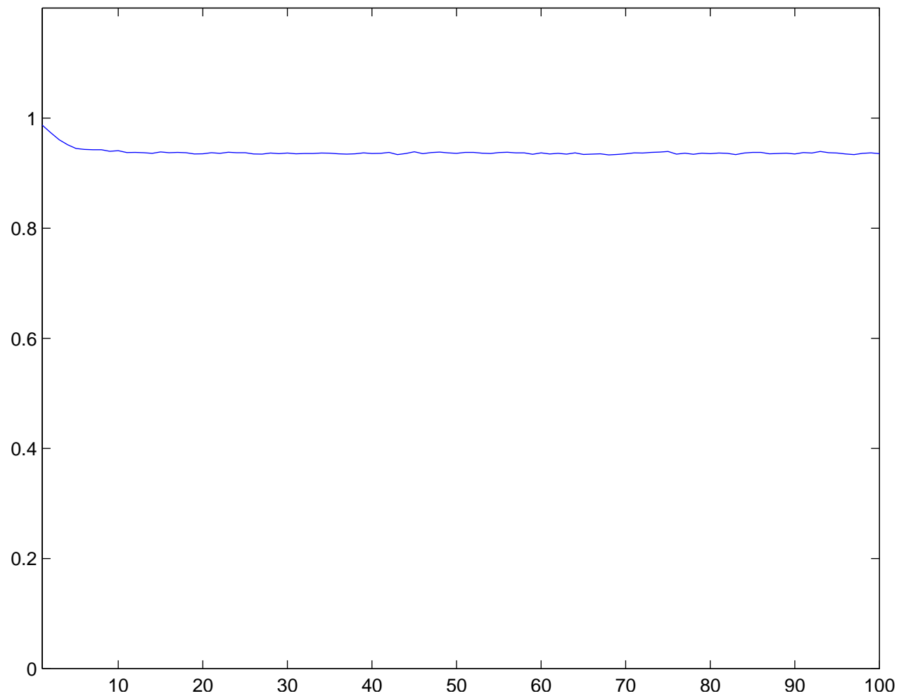
Individual run with N = 100 and \sigma = 2.25 averaged over 70 runs
