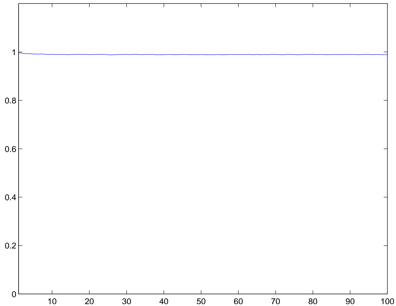
Individual run with N = 100 and \sigma = 1 averaged over 70 runs
