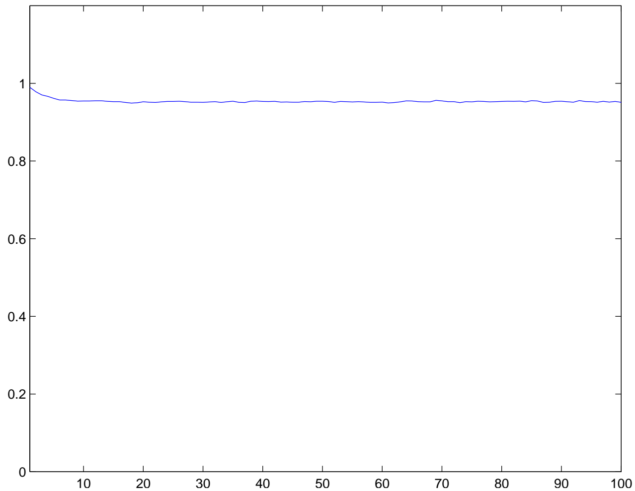
Individual run with N = 100 and \sigma = 2 averaged over 70 runs
