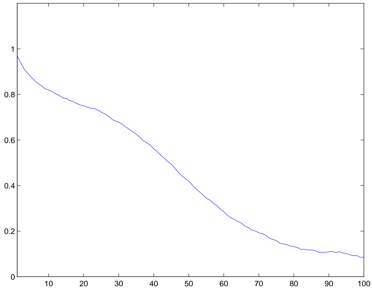
Individual run with N = 100 and \sigma = 3.25 averaged over 70 runs
