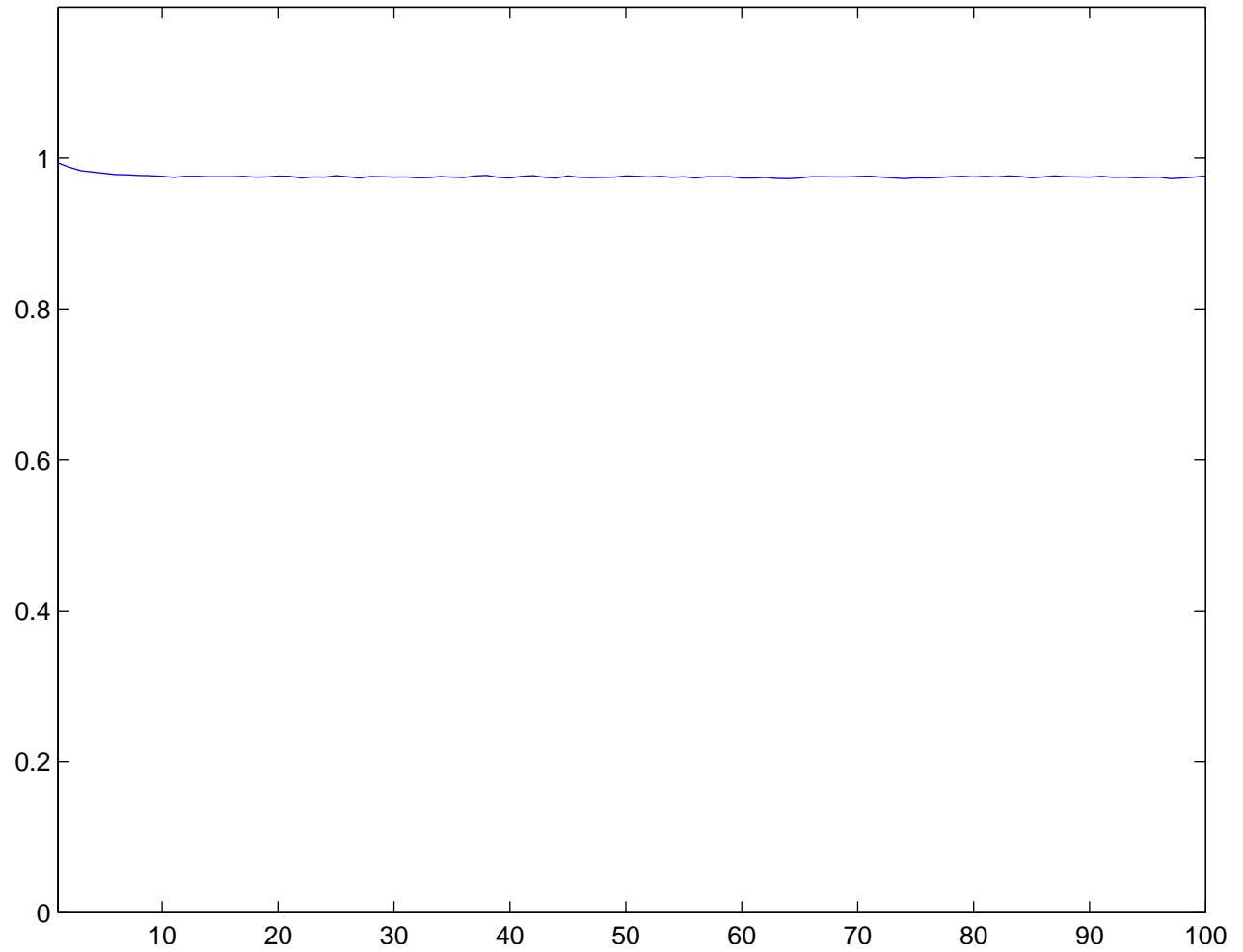
Individual run with N = 100 and \sigma = 1.5 averaged over 70 runs
