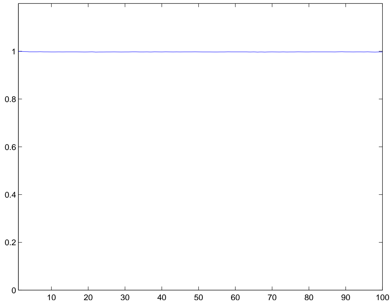
Individual run with N = 100 and \sigma = 0.5 averaged over 70 runs
