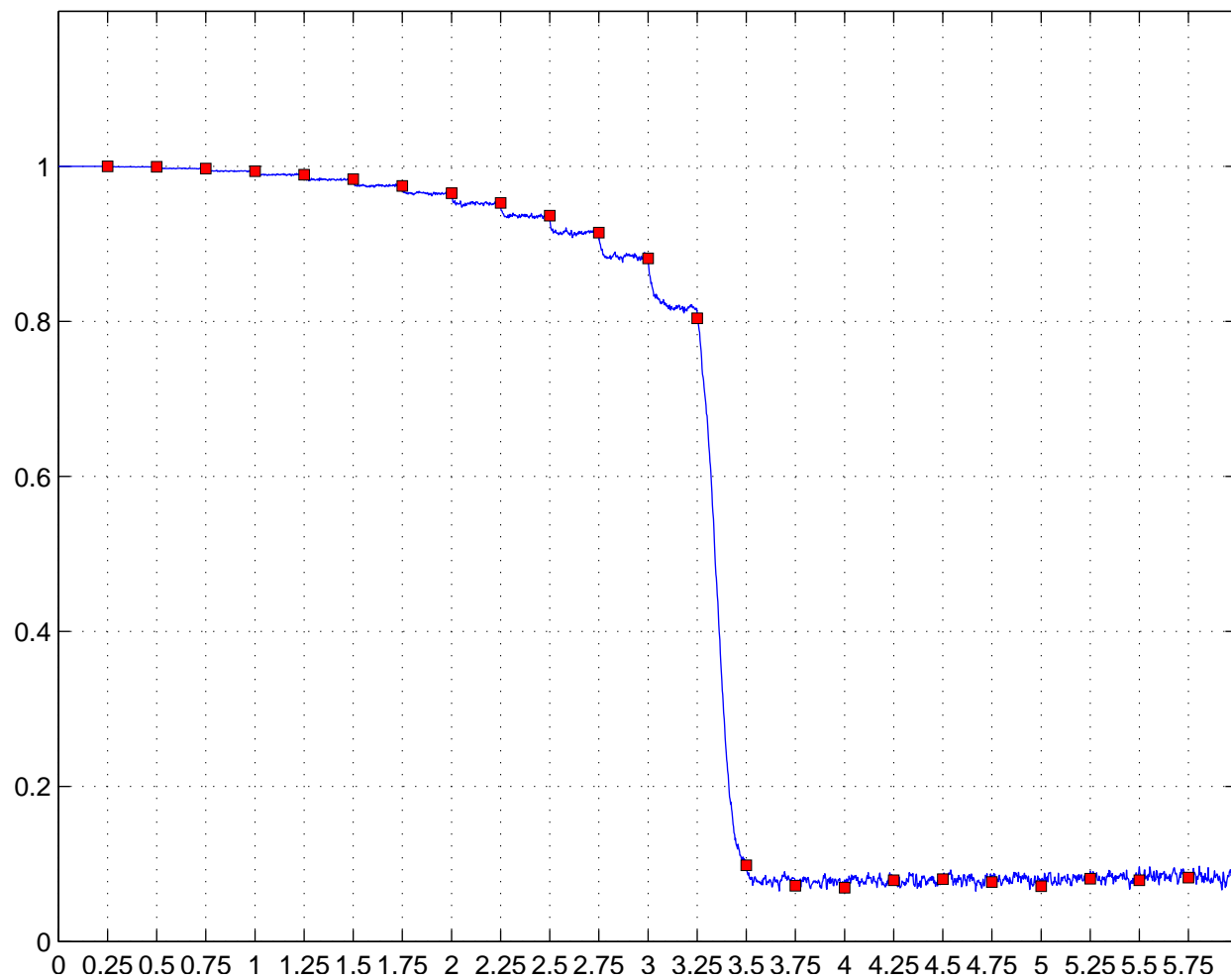
Run with N = 100 and sigma from 0 to 5.75 averaged over 70 runs
