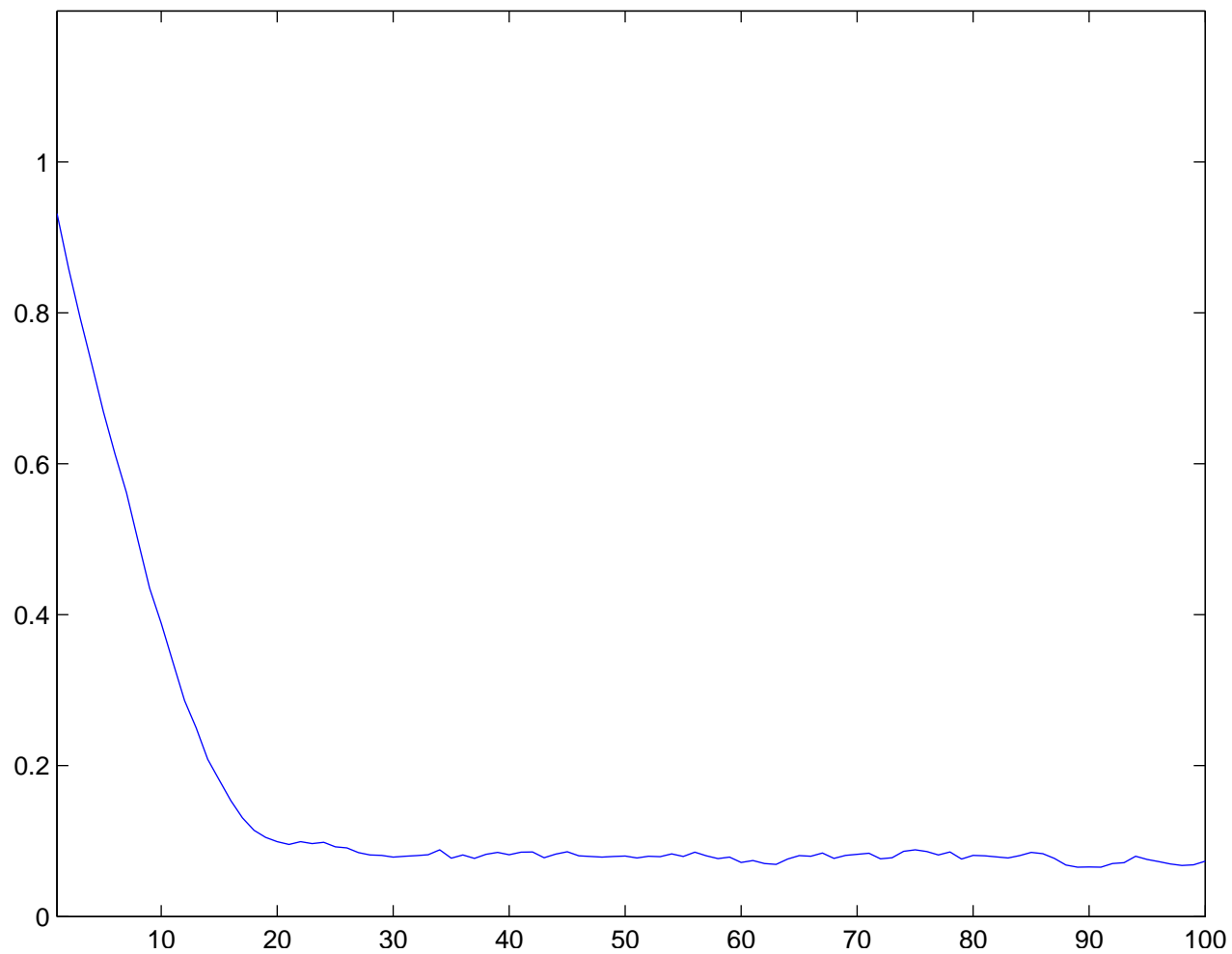
Individual run with N = 100 and \sigma = 4.75 averaged over 70 runs
