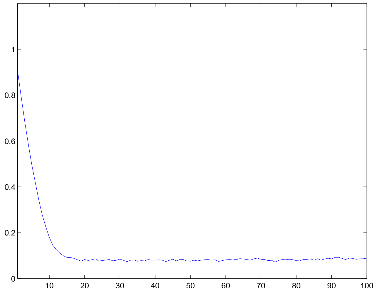
Individual run with N = 100 and \sigma = 5.75 averaged over 70 runs
