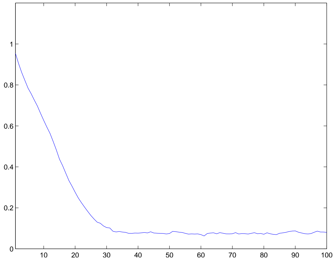
Individual run with N = 100 and \sigma = 4 averaged over 70 runs
