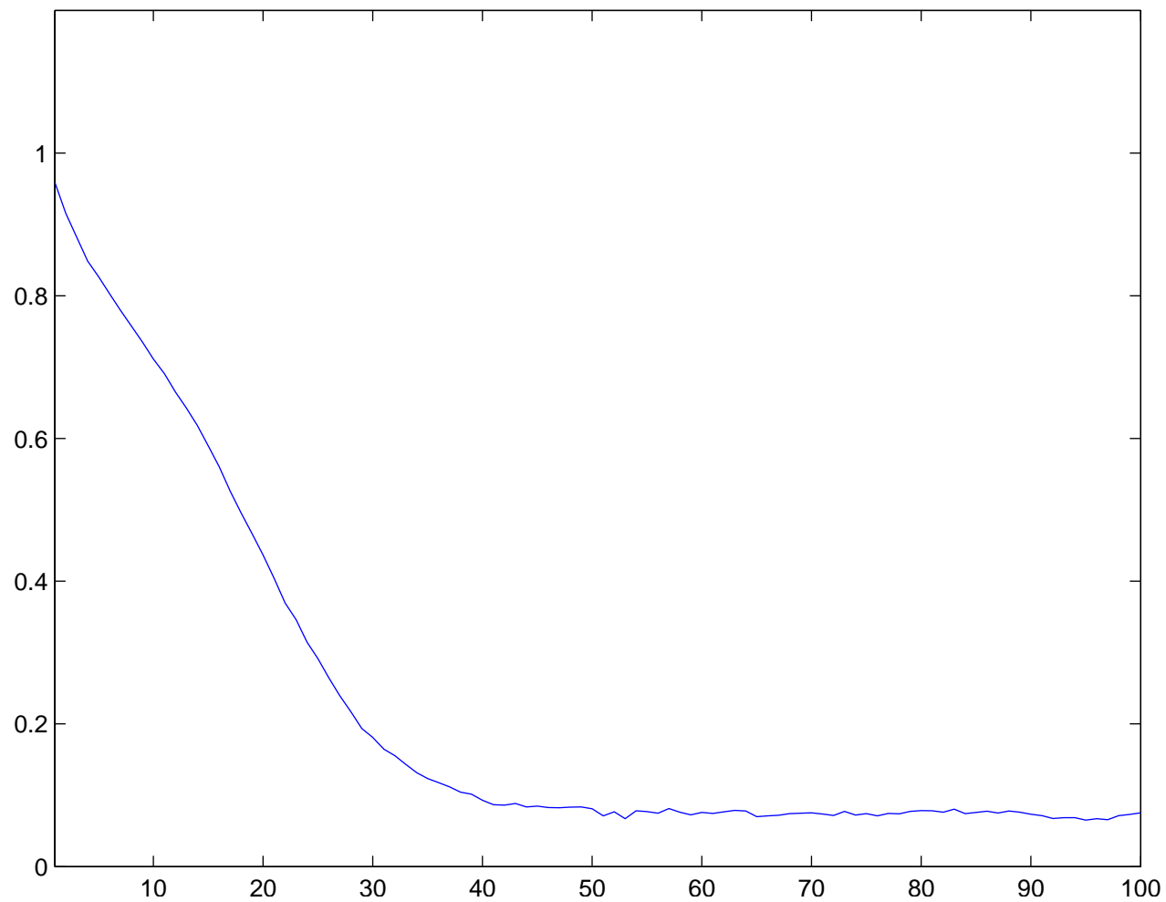
Individual run with N = 100 and \sigma = 3.75 averaged over 70 runs
