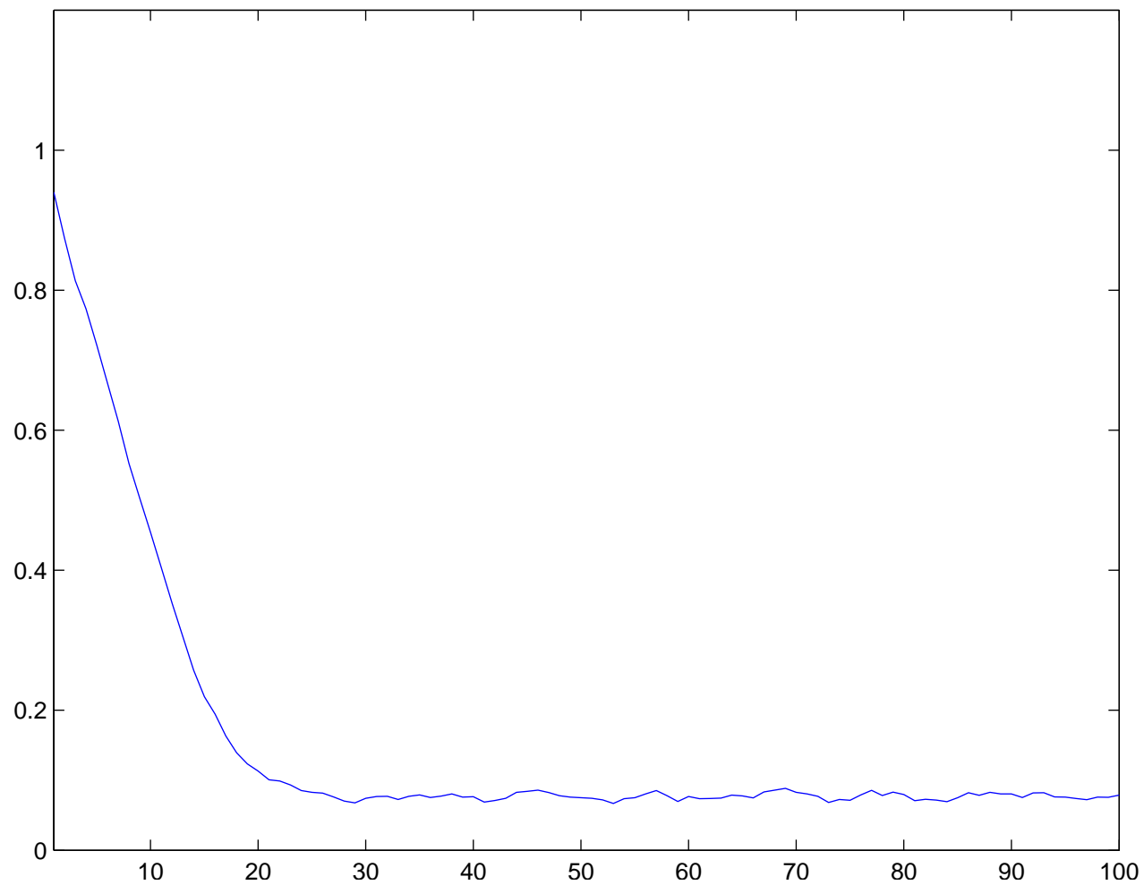
Individual run with N = 100 and \sigma = 4.5 averaged over 70 runs
