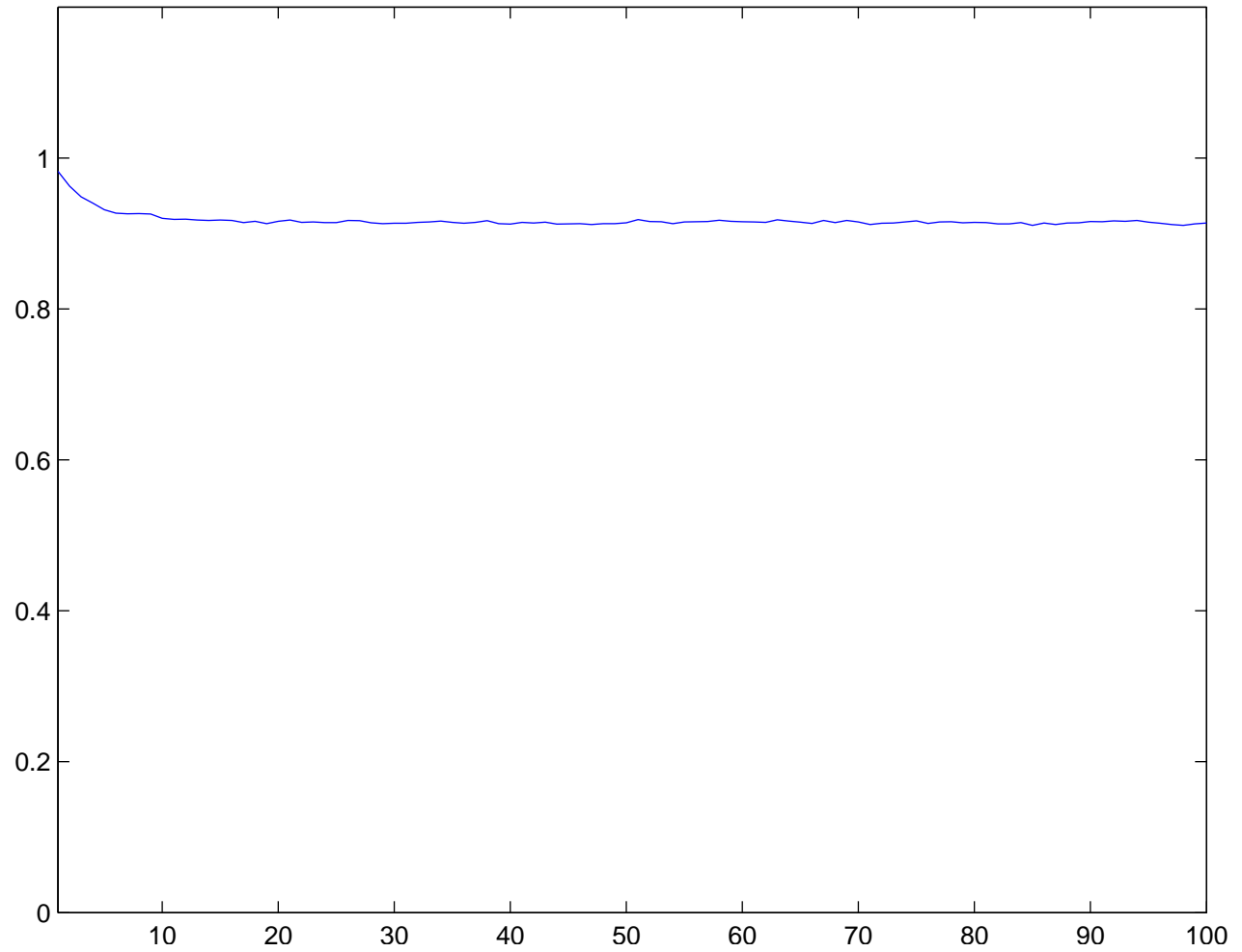
Individual run with N = 100 and \sigma = 2.5 averaged over 70 runs
