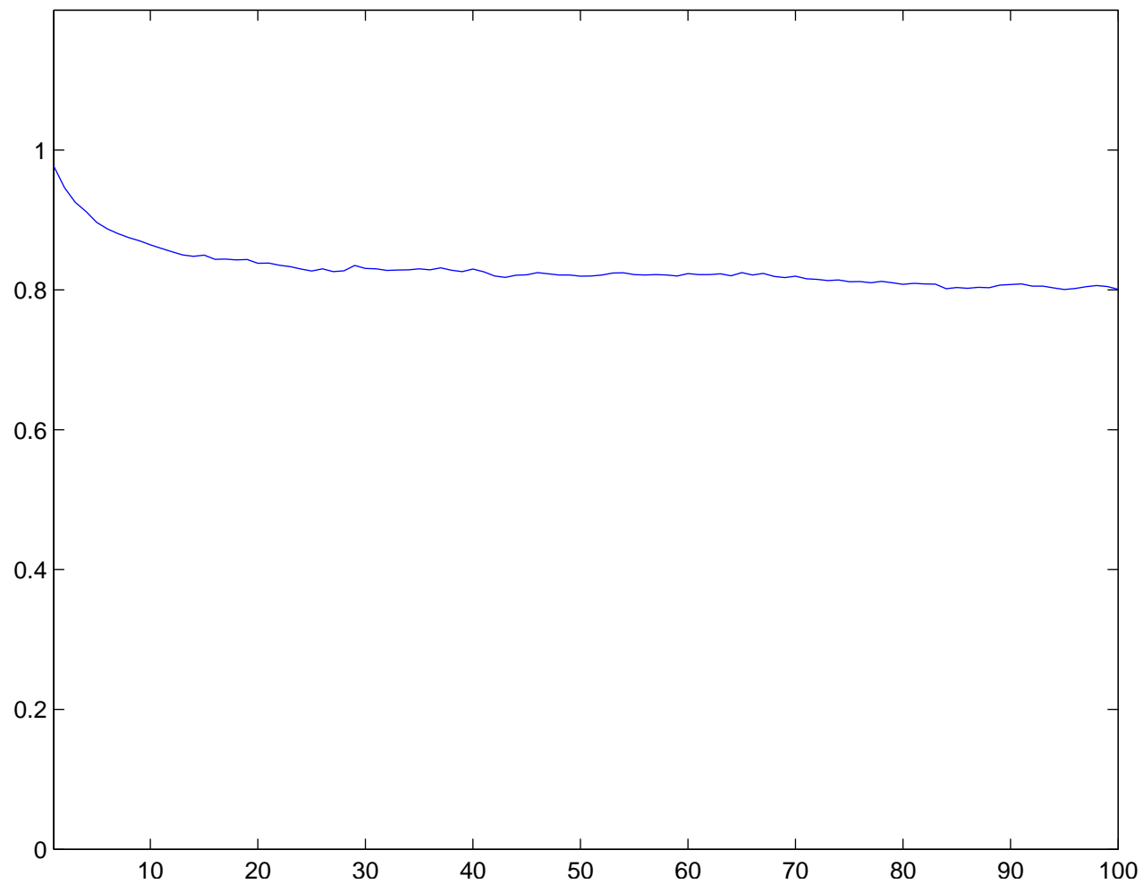
Individual run with N = 100 and \sigma = 3 averaged over 70 runs
