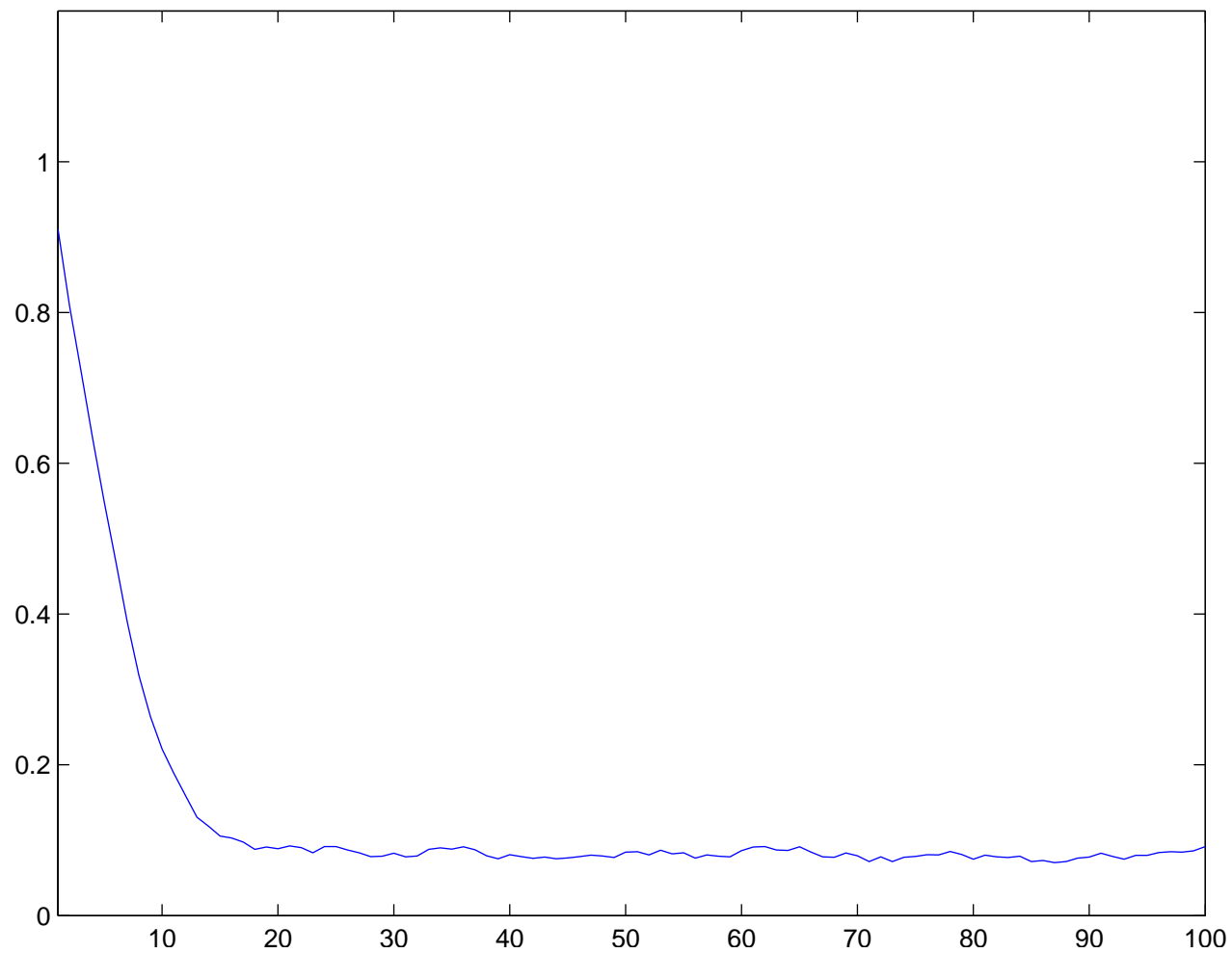
Individual run with N = 100 and \sigma = 5.5 averaged over 70 runs
