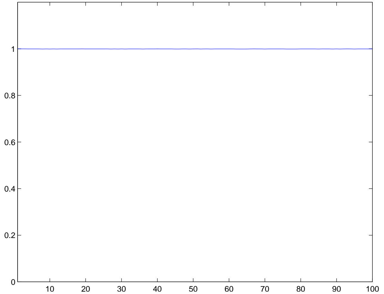
Individual run with N = 100 and \sigma = 0.25 averaged over 70 runs
