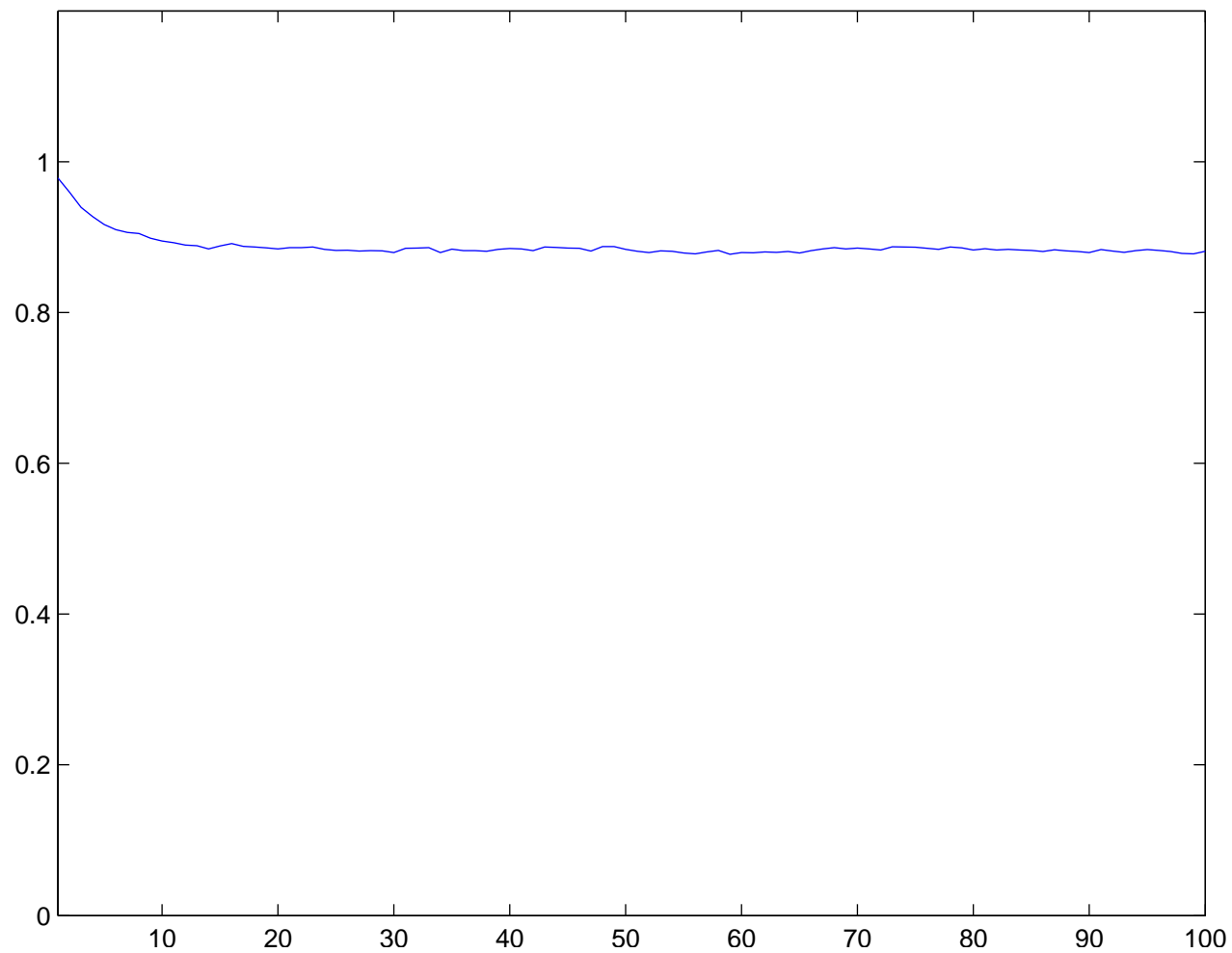
Individual run with N = 100 and \sigma = 2.75 averaged over 70 runs
