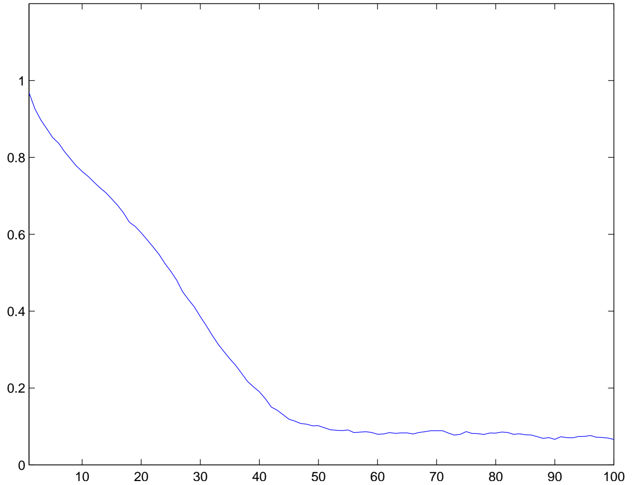
Individual run with N = 100 and \sigma = 3.5 averaged over 70 runs
