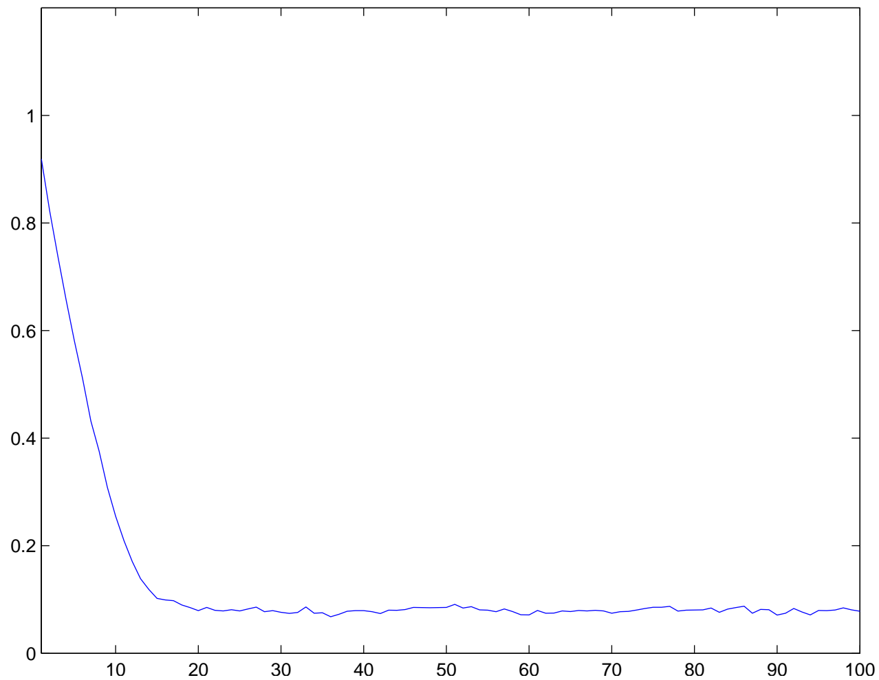
Individual run with N = 100 and \sigma = 5.25 averaged over 70 runs
