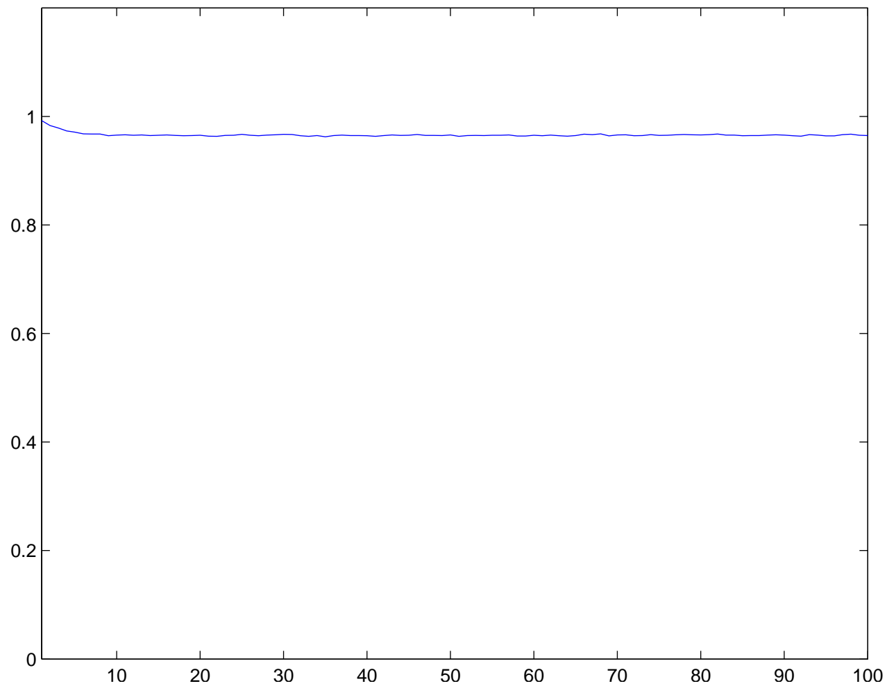
Individual run with N = 100 and \sigma = 1.75 averaged over 70 runs
