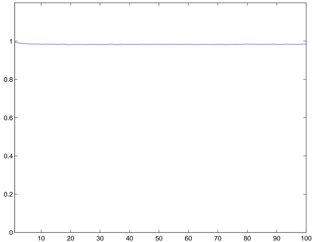
Individual run with N = 100 and \sigma = 1.25 averaged over 70 runs
