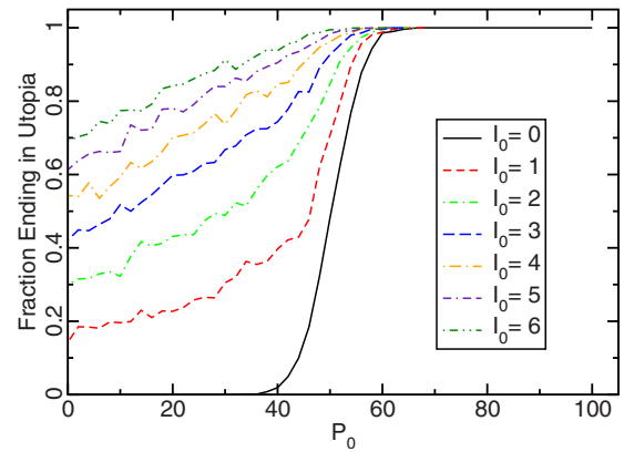
FIG. 3. (Color online) Even a small number of informants substantially increase the likelihood that a society will evolve toward utopia. Here, we plot the probability of the stochastic system ending in utopia given the initial numbers of paladins ( P_0 ) and informants ( I_0 ), assuming zero initial apathetics; higher I_0 values lead to greater probability of ending in utopia. Simulations used N=100 , M=5 , \delta=0.3 , \theta=0.6 , and \epsilon=0.2 , and were run 1000 times for each initial condition.
