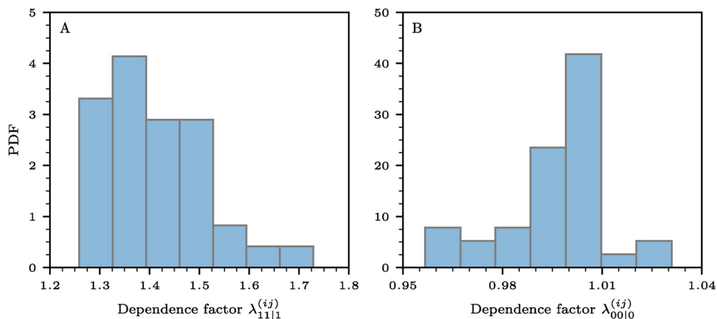
Fig 7. Probability density functions (PDFs) of dependence factors (A) \lambda_{11|1}^{(ij)} (see Eq (46)) and (B) \lambda_{00|0}^{(ij)} (see Eq (47)).
