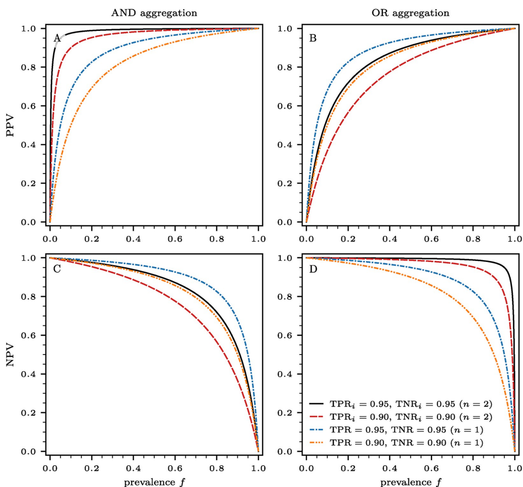
Fig 3. Positive predictive value (PPV) and negative predictive value (NPV) as a function of prevalence f . The results that we show in panels (A,C) and (B,D) are based on AND and OR aggregations of n = 2 tests, using Eqs (14) and (15), respectively. We denote the sensitivities and specificities of the two tests i \in \{1, 2\} by \text{TPR}_i and \text{TNR}_i , respectively. We consider two different combinations of true positive and true negative rates (solid black lines: \text{TNR}_i = 0.95 and \text{TNR}_i = 0.95 ; dashed red lines: \text{TNR}_i = 0.90 and \text{TNR}_i = 0.90 ). As a reference, we also show results for single tests without further aggregation (dash-dotted blue line: \text{TNR} = 0.95 and \text{TNR} = 0.95 ; dash-dot-dotted orange line: \text{TNR} = 0.90 and \text{TNR} = 0.90 ). These curves are independent of the ordering (parallel or series) method used.
