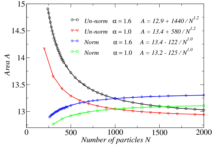
FIGURE 2.1. Area of unidirectional milling structures as a function of particle number N . The upper curve represents the unnormalized potentials, the lower one the potential normalized so that the total mass is kept at M = Nm = 1000 . Milling parameters are chosen as C_a = 0.5 , C_r = 1.0 , \ell_a = 3 , \ell_r = 0.5 while the self-propulsion terms are set at \alpha = 1.6 , \beta = 0.5 and at \alpha = 1.0 , \beta = 0.5 . The normalized and unnormalized curves match at N = 1000 , which is the reference point for the unnormalized potential. Curves can be fitted as A \sim A_0 + B/N^\xi , where \xi = 1.2 or \xi = 1.0 for the unnormalized and normalized potentials, respectively.
