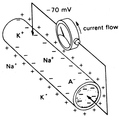
Figure 5.1 Resting, or membrane potential. Sodium ( \text{Na}^+ ) ions are in high concentration outside the membrane, while potassium ( \text{K}^+ ) ions and organic anions ( \text{A}^- ) are in high concentration inside the membrane. The potential across the membrane is about -70 millivolts.
