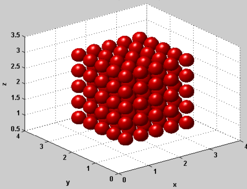
NaCl(fcc Structure)
