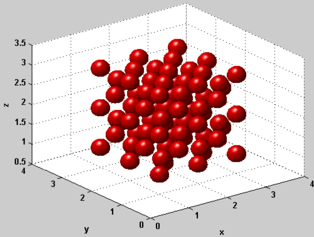
Carbon(Diamond Structure)
