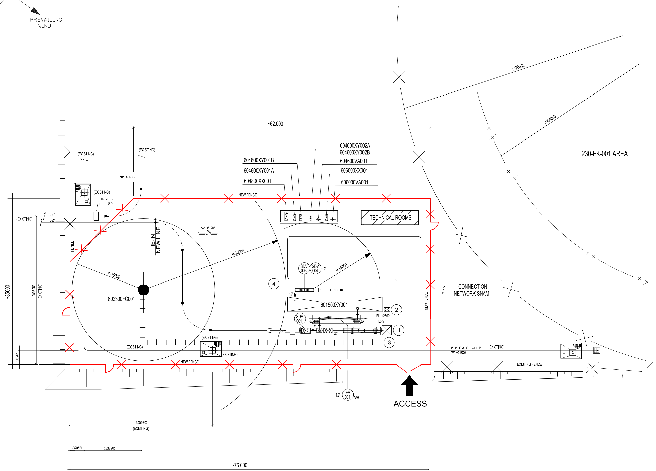
PLOT PLAN
